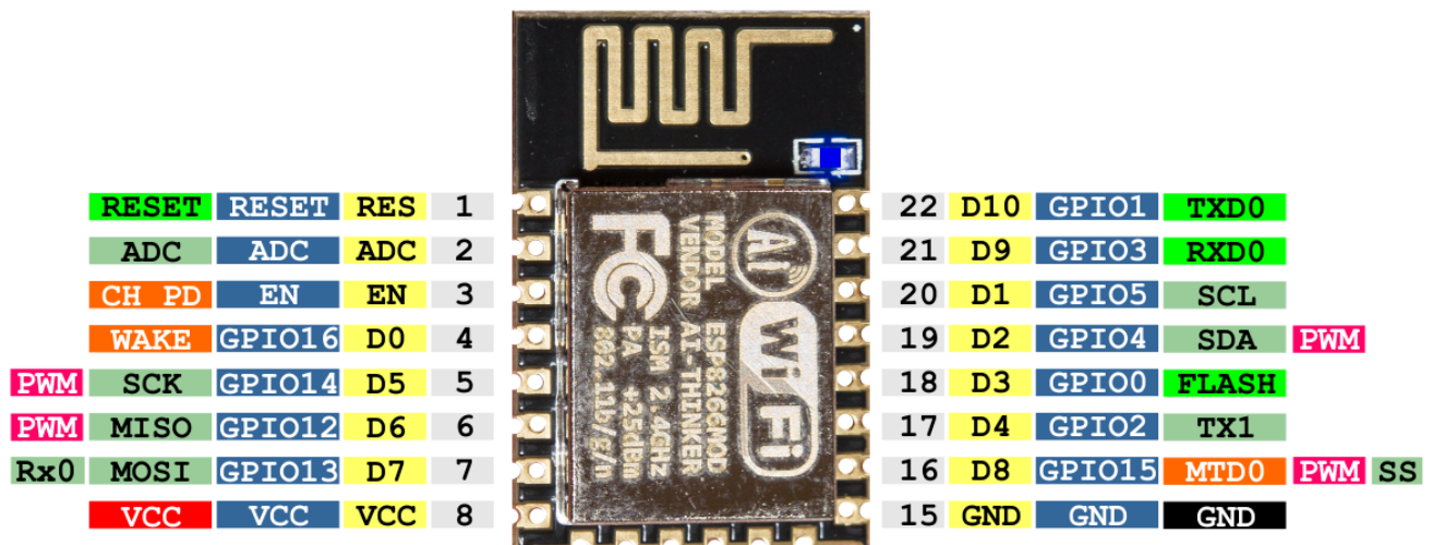
ESP-12F Alternate Functions Map:
