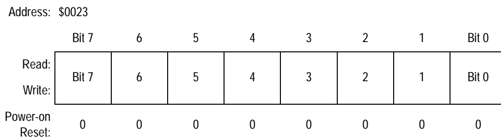
Figure 18-13. Breakpoint Address Register Low (BRKAL)
