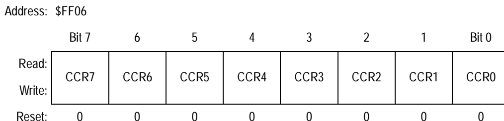
Figure 18-9. BDM CCR Holding Register (CCRSV)
