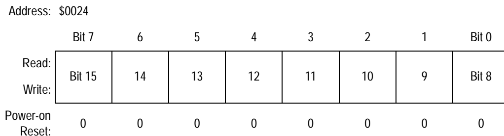
Figure 18-14. Breakpoint Data Register High (BRKDH)
